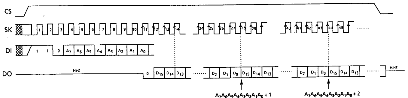
Figure 6 Read Timing (S-29U330A)
